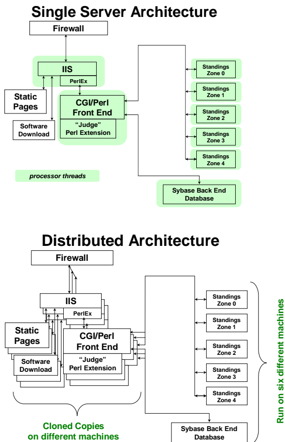
Figure 3. Scalable Services Architecture for the Contest Server.
