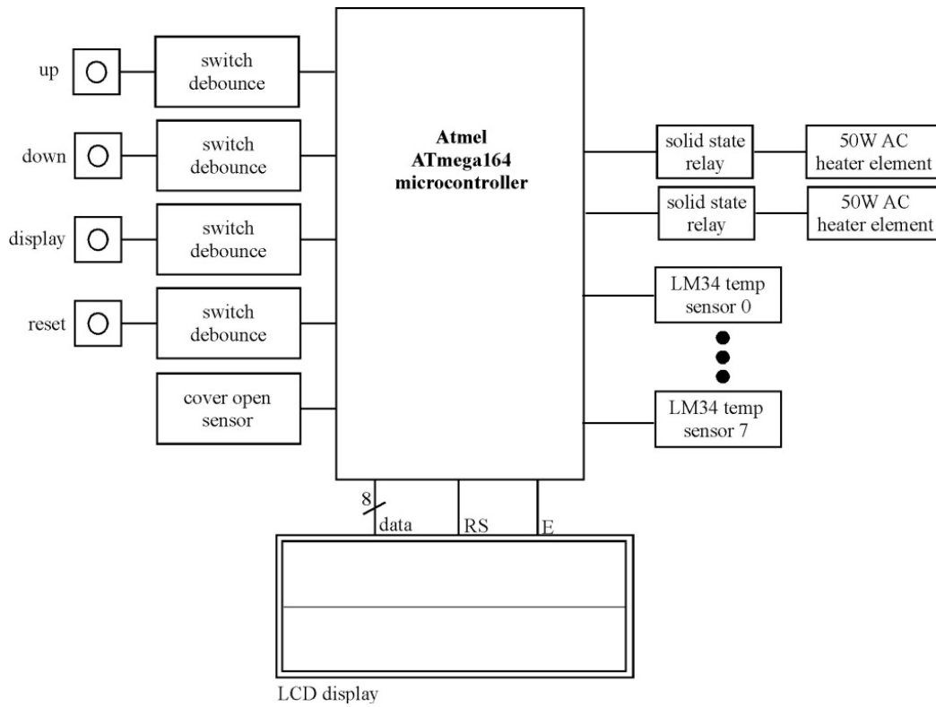
Figure 3. Concrete Curing Box (CCB) interface diagram.
