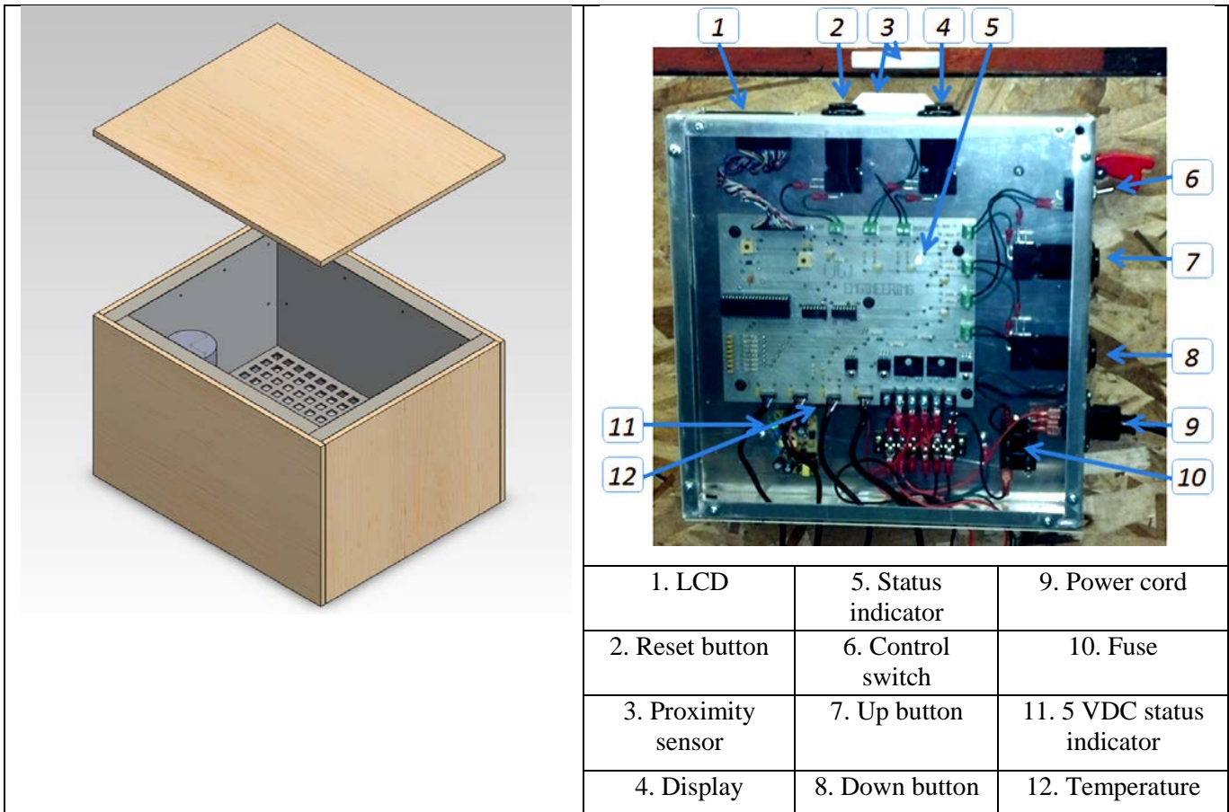
Figure 6. Overall design: (left) heating chamber and (right) control panel.
