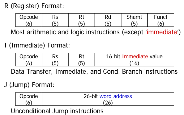
Figure 2. Instruction formats for MIPS architecture [1]
