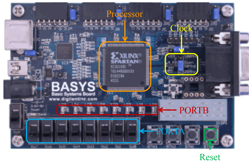
Figure 12: FPGA Implementation of Microcontroller.
