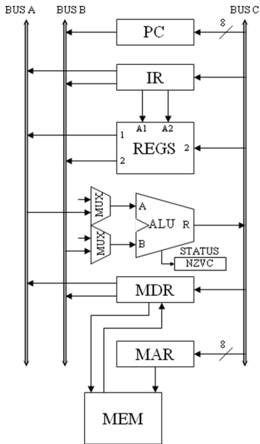
Figure 1: Data Path for Instructional Processor.
