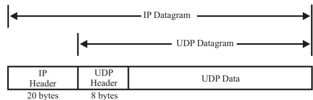
Figure 5: UDP encapsulation.
